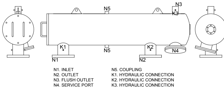
180 SERIES FILTER - GENERAL LAYOUT
