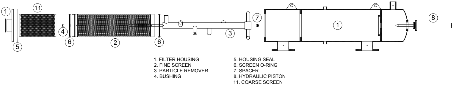
180 SERIES FILTER - EXPLODED VIEW
