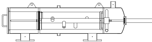
180 SERIES FILTER - ASSEMBLED VIEW
